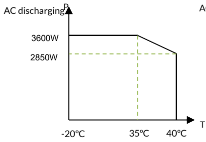
AC discharging power Vs temperature
