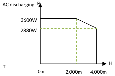
AC discharging power Vs altitude
